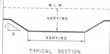
TYPICAL SECTION
